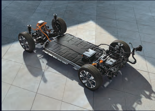
Electric Global Modular Platform (E-GMP) The New E-GMP platform introduces a flat floor, facilitating comfort and utility along with greater power, driving range and control
